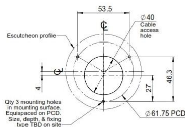
MOUNTING HOLE DETAILS Dimensions in mm
