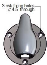
MOUNTING SEAT & ESCUTCHEON COVER Dimensions in mm
