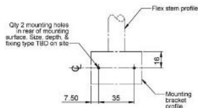
MOUNTING HOLES Dimensions in mm
