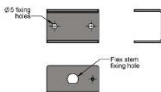
MOUNTING BRACKET Dimensions in mm
